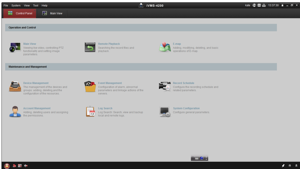
Figure 3. 2 Main Interface
