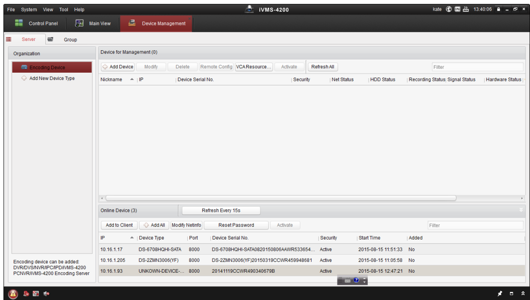
Figure 3. 3 Device Management
